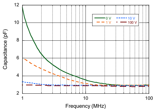
Capacitance vs. Frequency & Reverse Voltage (MA4PK2000 Series)
