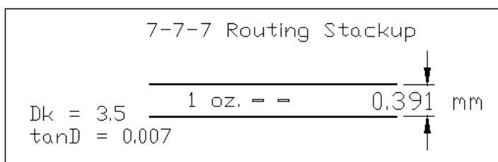
Figure 13: 7-7-7 Routing
