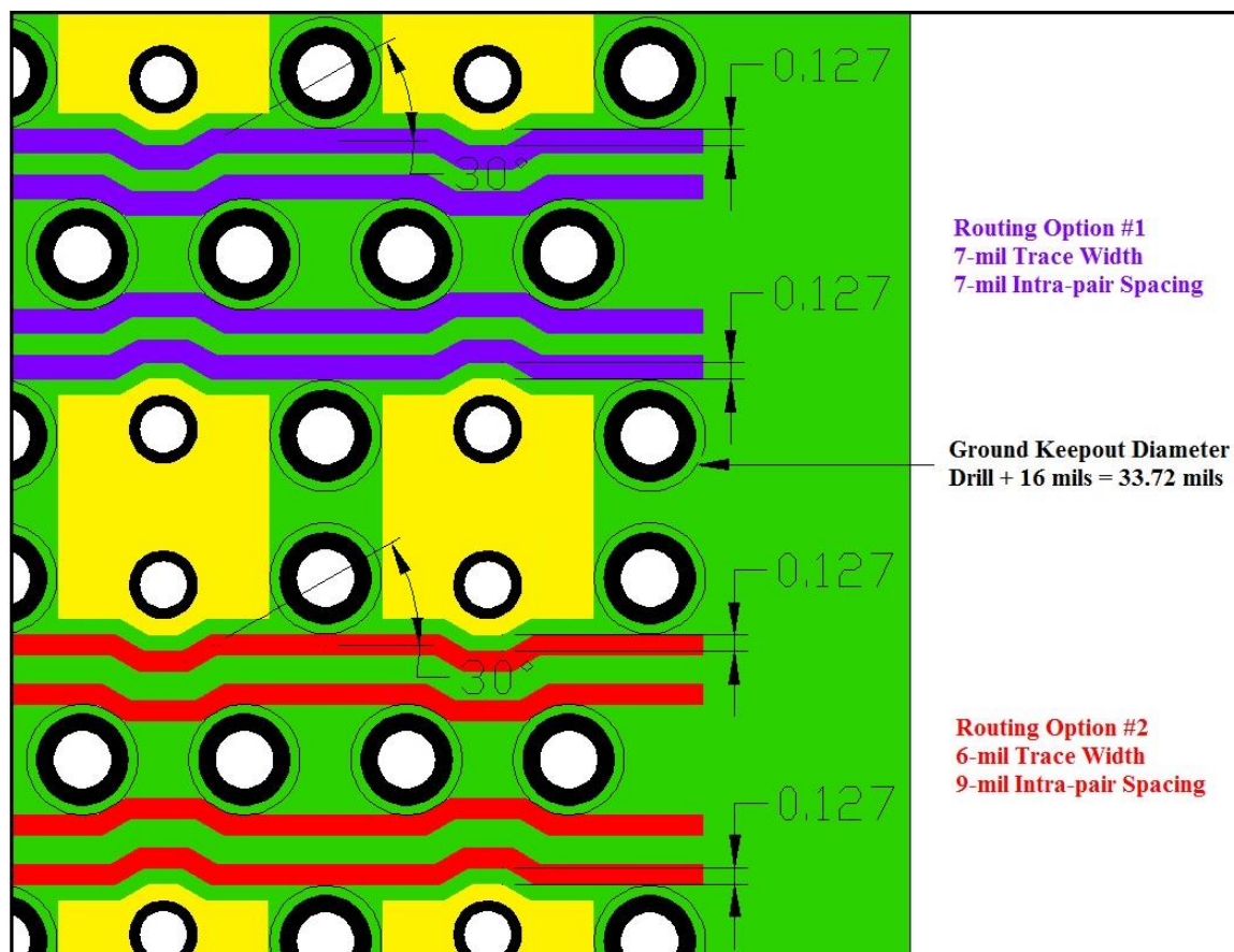
Figure 8: Daughtercard Channel Routing
