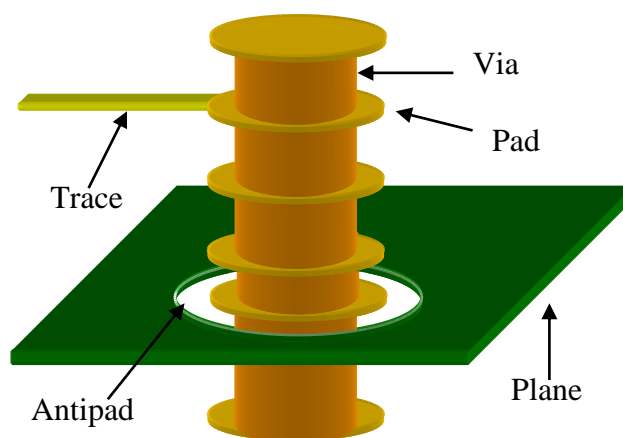
Figure 3: Antipad Illustration
