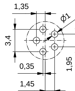
Pin layout PCB
