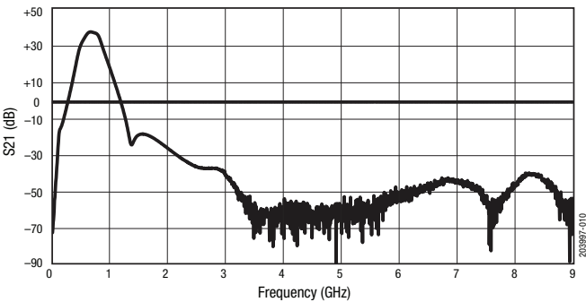
Figure 10. S21 vs Frequency
