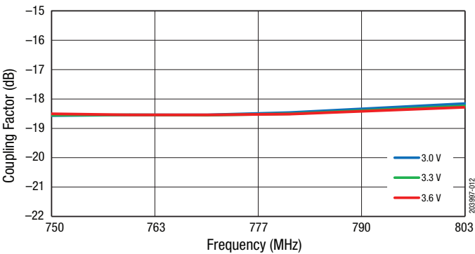
Figure 12. Coupling Factor vs Frequency Across Power Supply
