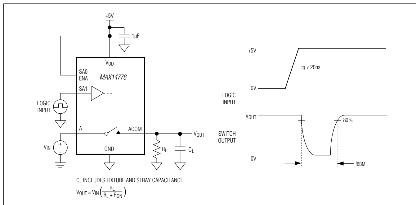
Figure 4. Break-Before-Make Timing
