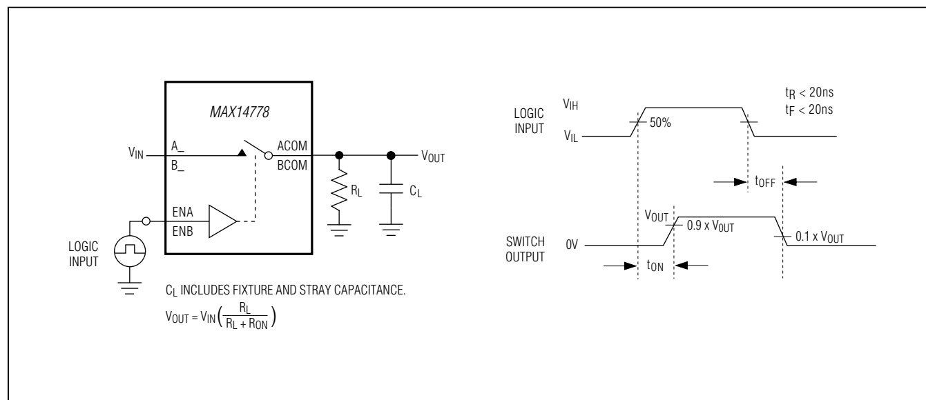
Figure 3. Turn-On/Turn-Off Timing
