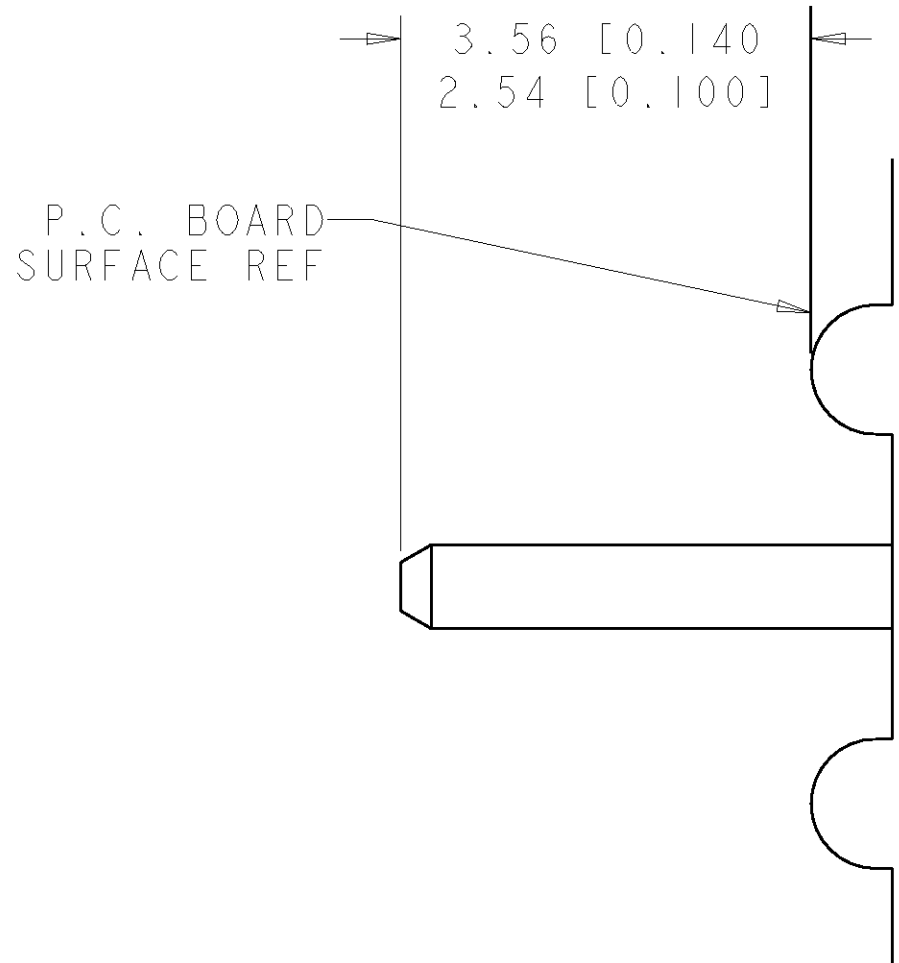
6. SOLDER PIN DETAIL SCALE 10 : 1
