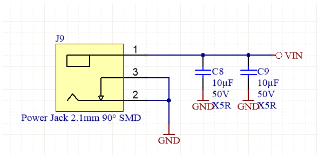
Figure 3: Power Connector
