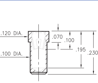
9801-0-15-XX-23-XX-10-0 Solder mount in .102 min. mounting hole
