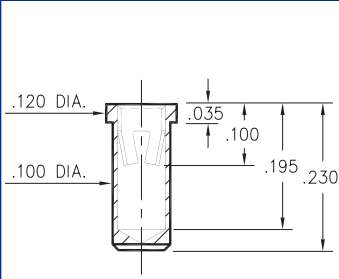
9401-0-15-XX-23-XX-10-0 Solder mount in .102 min. mounting hole
