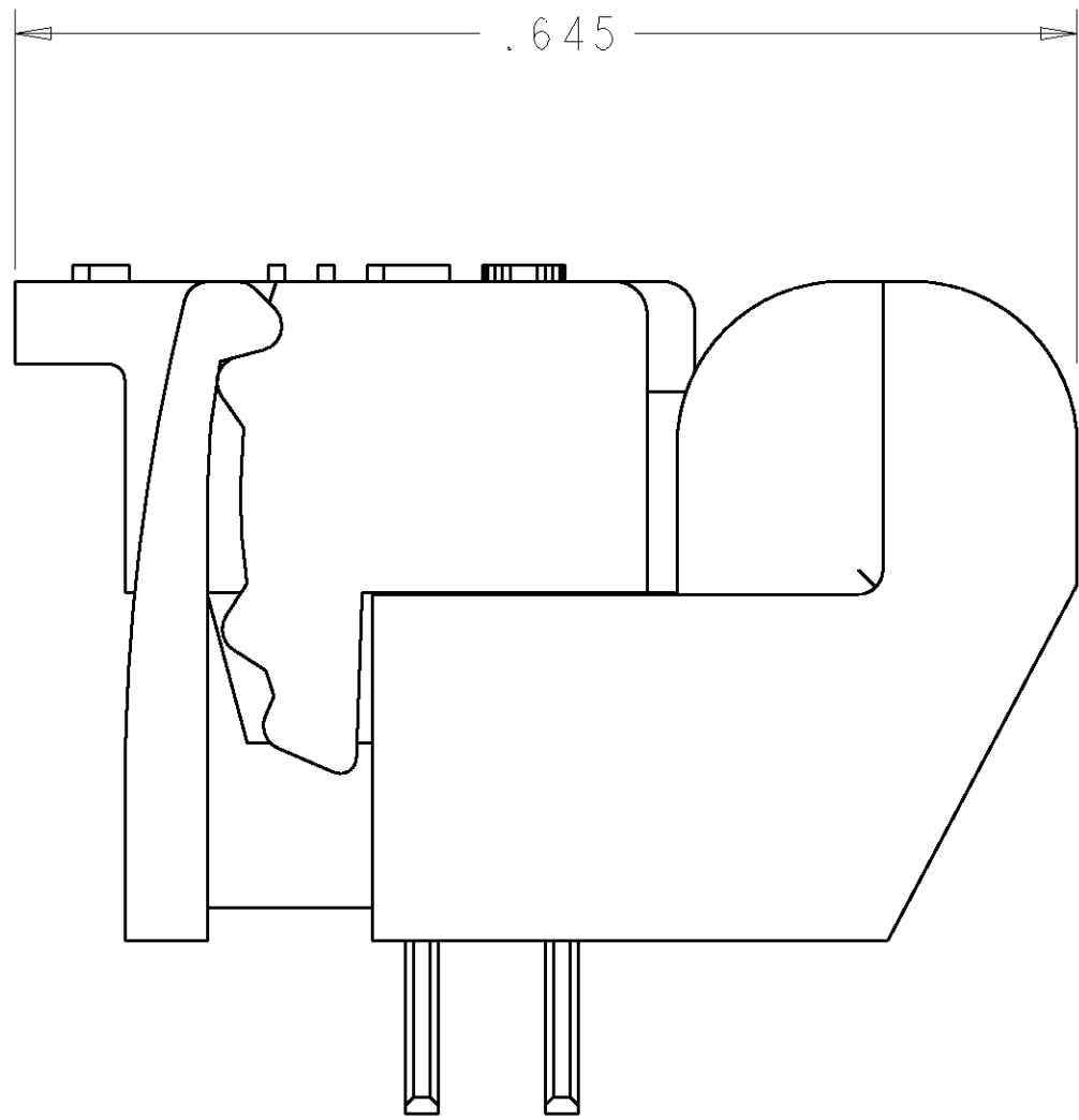
CLOSED POSITION
