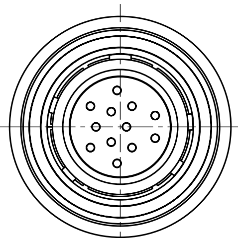
S12YDR-PDMXFGO-0000 Mechanical coding: D Color coding: green
