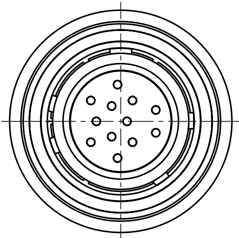
S12YCR-PDMXFGO-0000 Mechanical coding: C Color coding: blue
