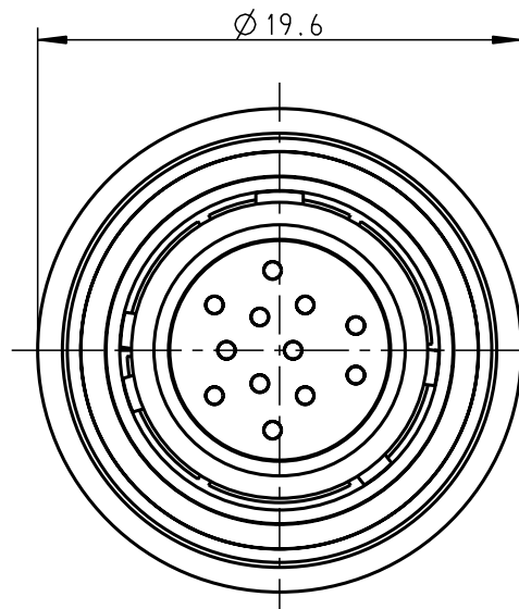
S12YAR-PDMXFGO-0000 Mechanical coding: A Color coding: light brown
