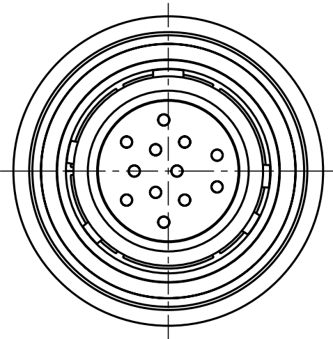
S12YBR-PDMXFGO-0000 Mechanical coding: B Color coding: red
