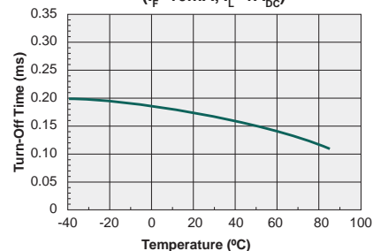
Typical Turn-Off Time vs. Temperature ( I_F=10\text{mA} , I_L=1\text{A}_{DC} )
