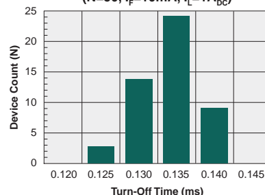
Typical Turn-Off Time (N=50, I_F=10\text{mA} , I_L=1\text{A}_{DC} )
