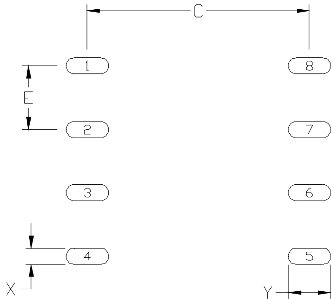
Figure 22. DIP8 Land Pattern
