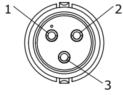
WIRE VIEW 6282-3PG-5XX
