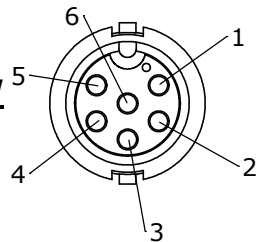
FACE VIEW 6282-6PG-5XX
