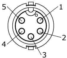
FACE VIEW 6282-5PG-5XX
