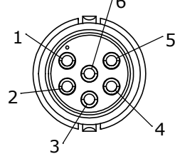
WIRE VIEW 6282-6PG-5XX
