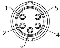
WIRE VIEW 6282-5PG-5XX
