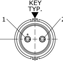
WIRE VIEW 6282-2PG-5XX
