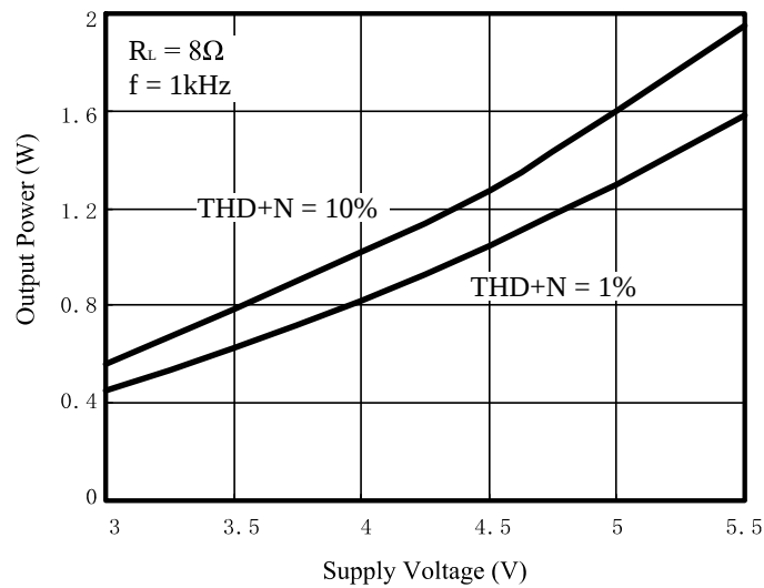
Figure 22 Output Power vs. Supply Voltage
