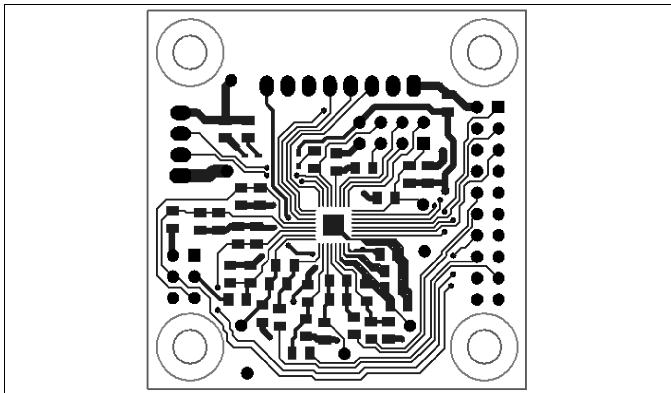
Figure 10 Top layer routing of the EVAL-M1-099M
