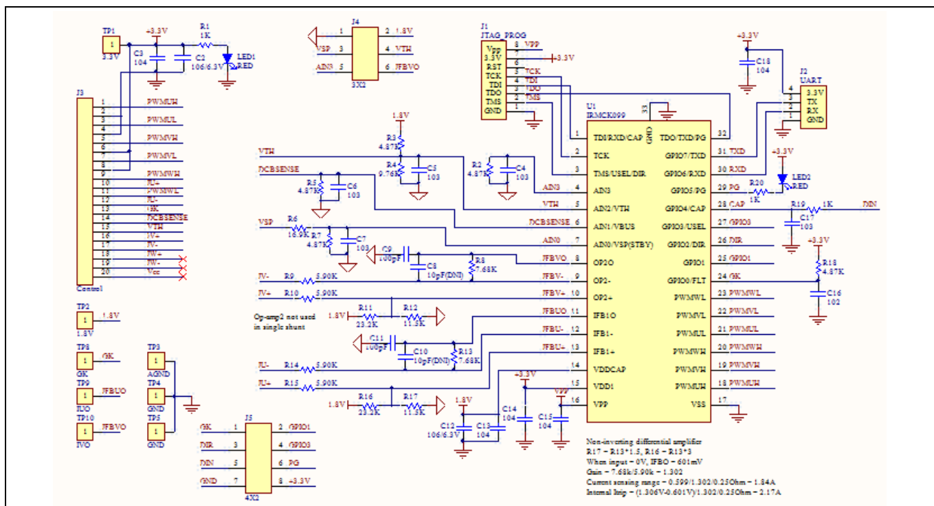
Figure 5 The schematics for the Eval-M1-099M evaluation board
