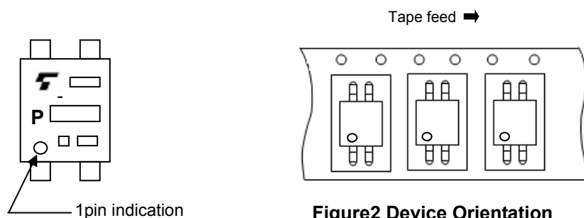
Figure2 Device Orientation
