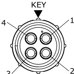
WIRE VIEW 5182-4PG-5XX
