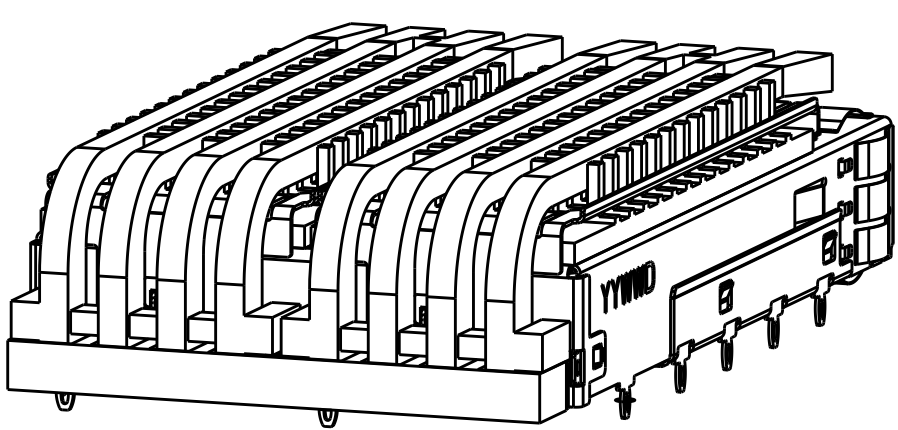
2170826-1 AS SHOWN SCALE 2:1
