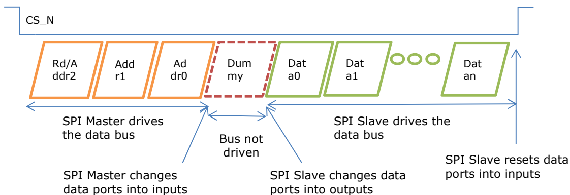
Figure 4-1 SPI master and slave in the master read case
