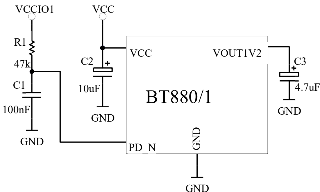
Figure 4-10 Internal regulator
