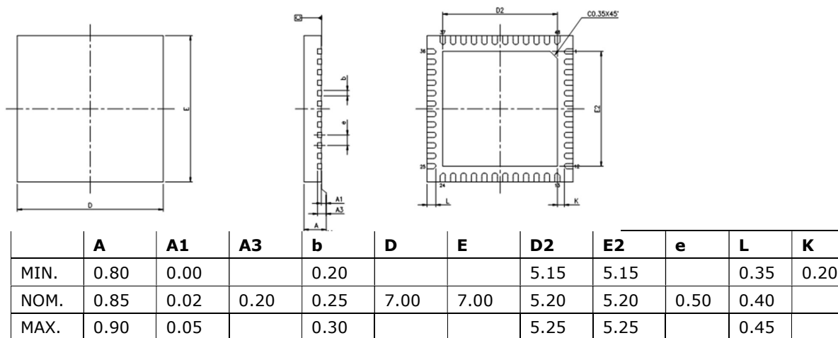
Figure 8-2 VQFN-48 Package Dimensions
