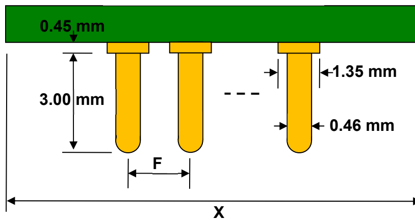
Side View (PGA Pins)
