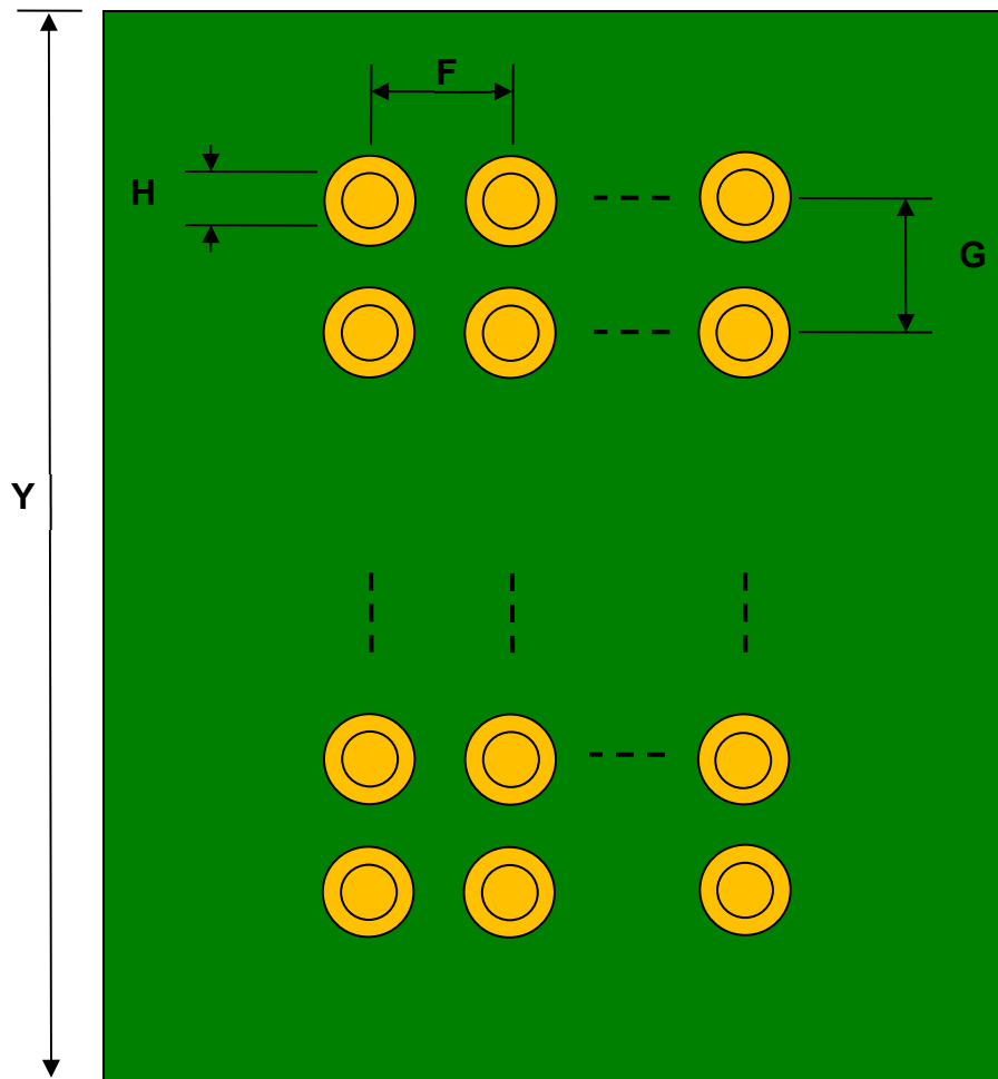
Bottom View (PGA Pins)
