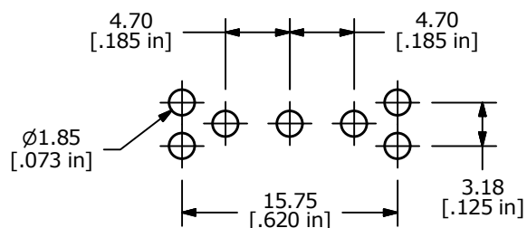
P.C. MOUNTING
