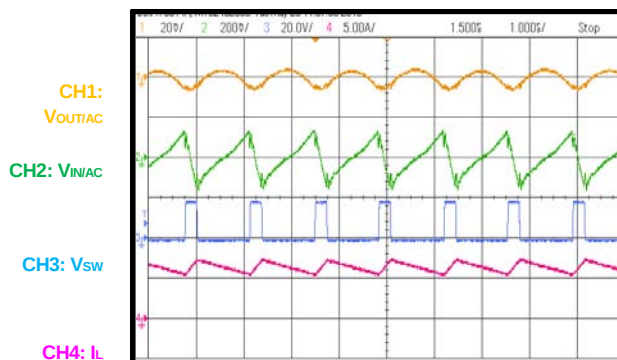
Input/Output Ripple I_{OUT} = 6.5A
