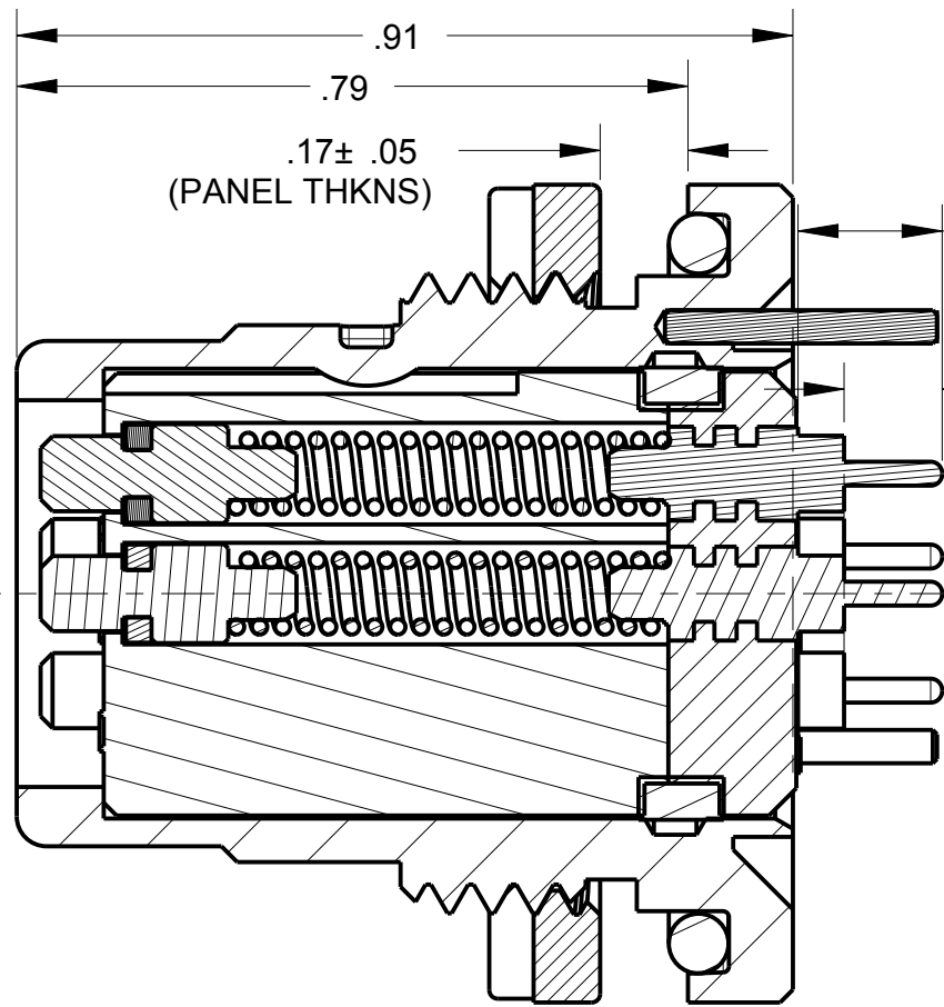
SECTION Z-Z SCALE 4.000
