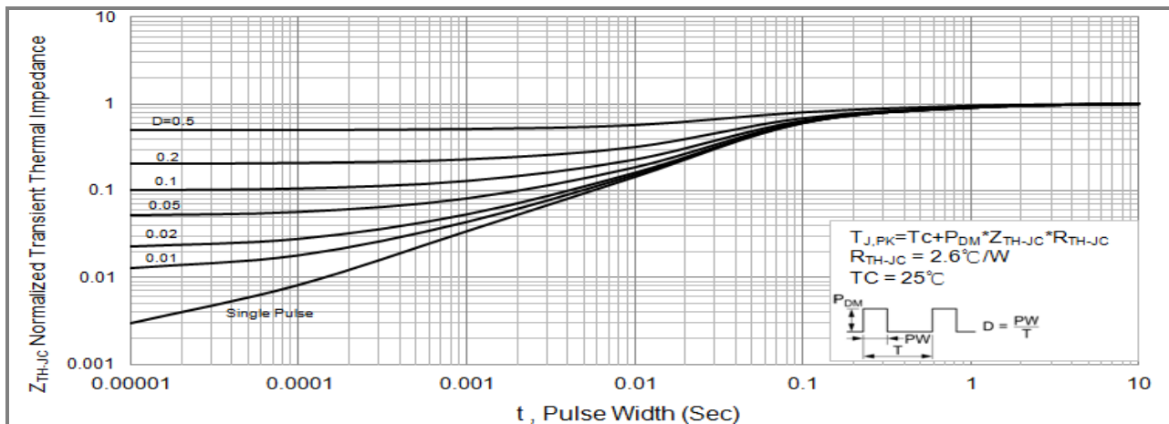
Fig.15 PJF5NA80 Normalized Transient Thermal Impedance vs. Pulse Width
