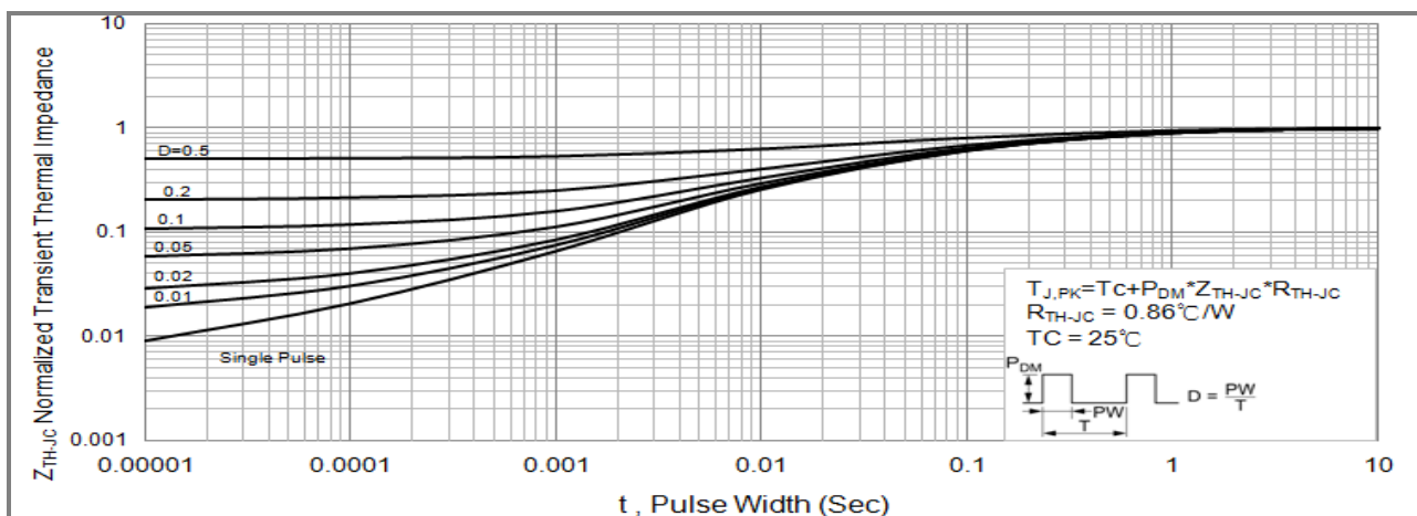
Fig.14 PJP5NA80 Normalized Transient Thermal Impedance vs. Pulse Width
