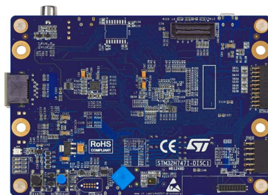
STM32H747I-DISCO1 (top view)
