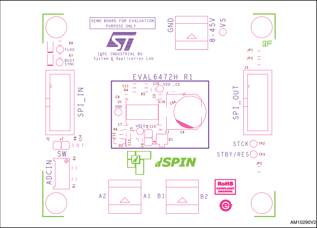
Figure 3. EVAL6472H - silkscreen
