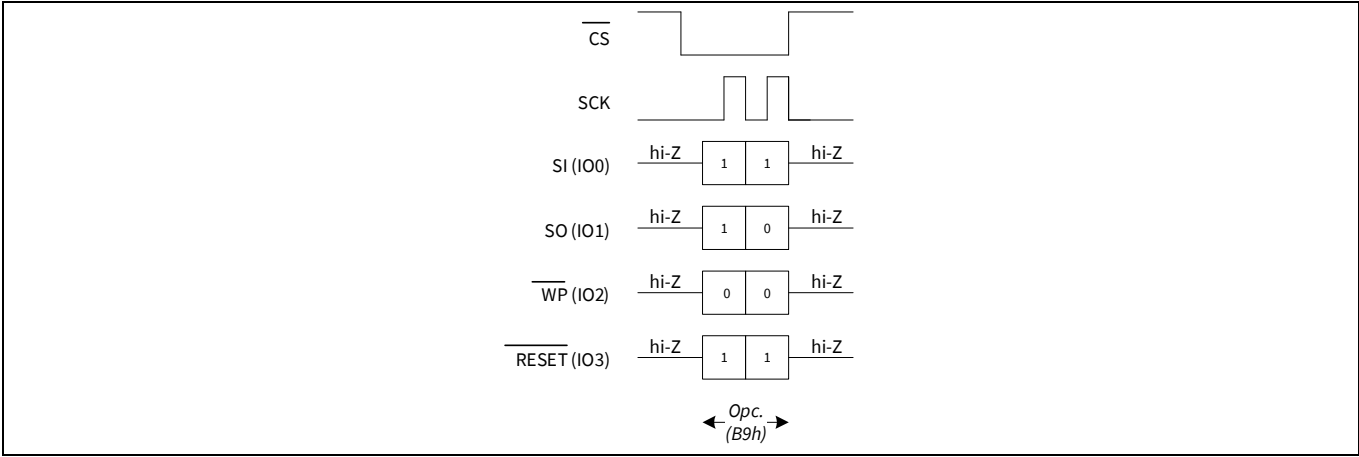
Figure 102 Deep power-down mode operation in QPI mode
