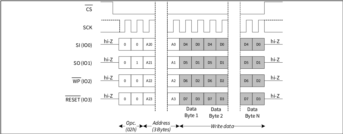
Figure 42 Memory write (WRITE) in QPI mode
