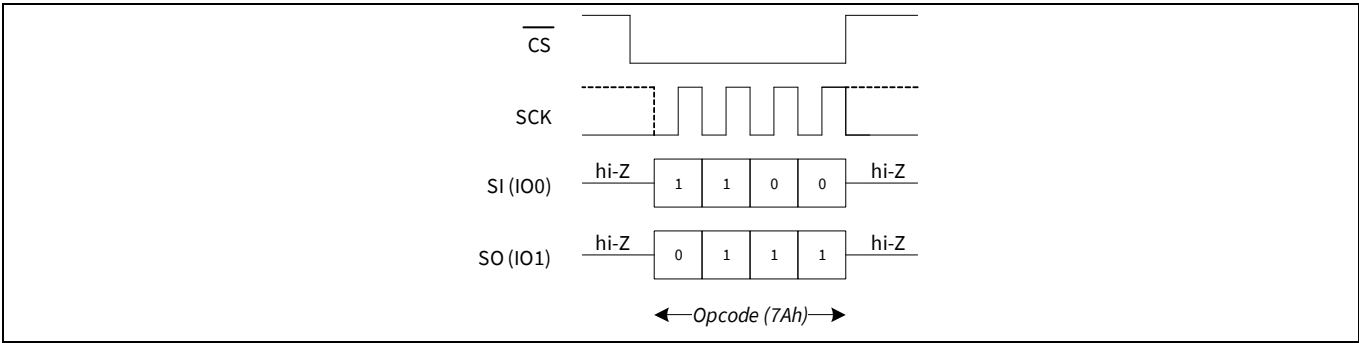
Figure 86 CRC resume (EPCR) in DPI mode
