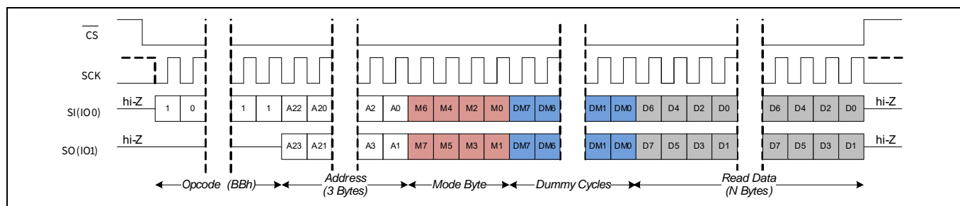
Figure 61 Double I/O read (DIOR)
