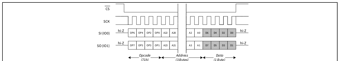
Figure 35 Write any register (WRAR) in DPI mode
