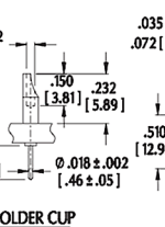
③ SOLDER CUP
