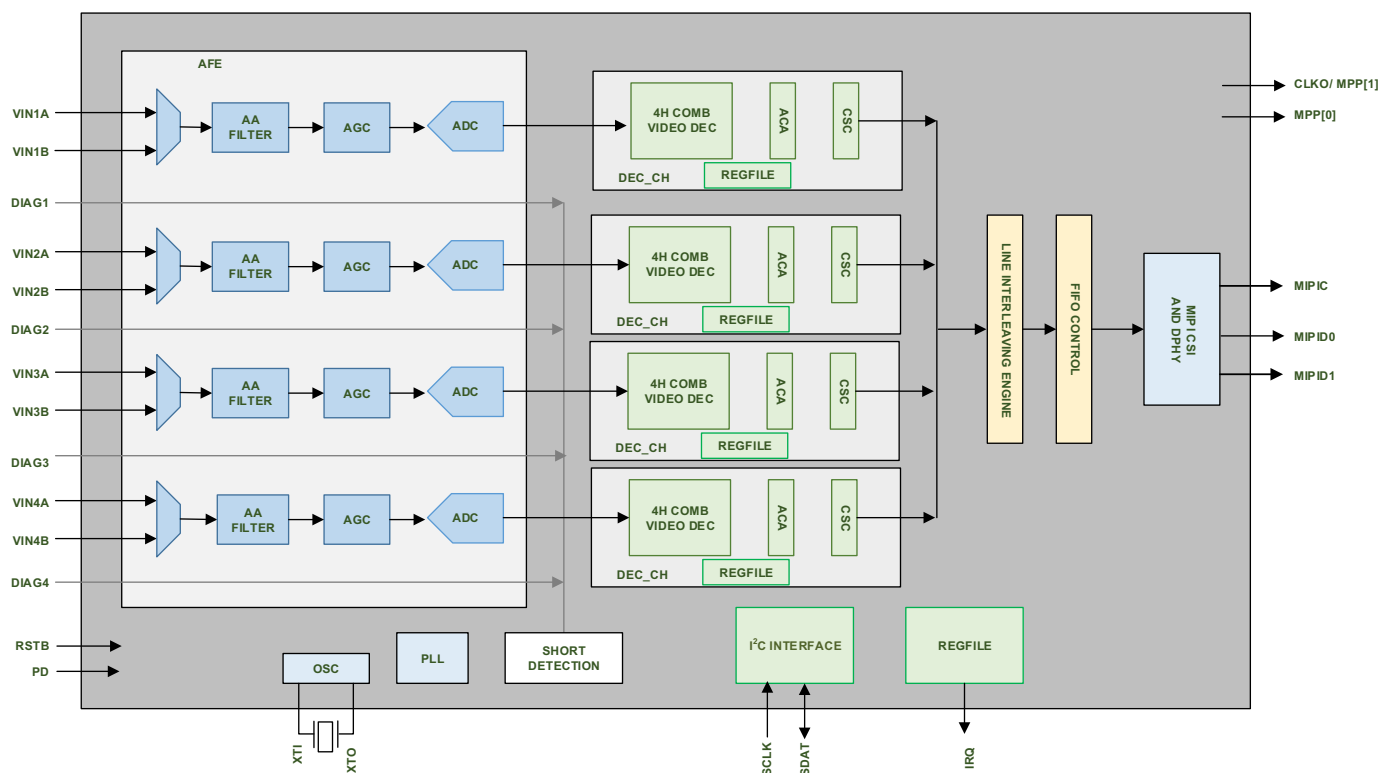
FIGURE 1. ISL79985 BLOCK DIAGRAM
