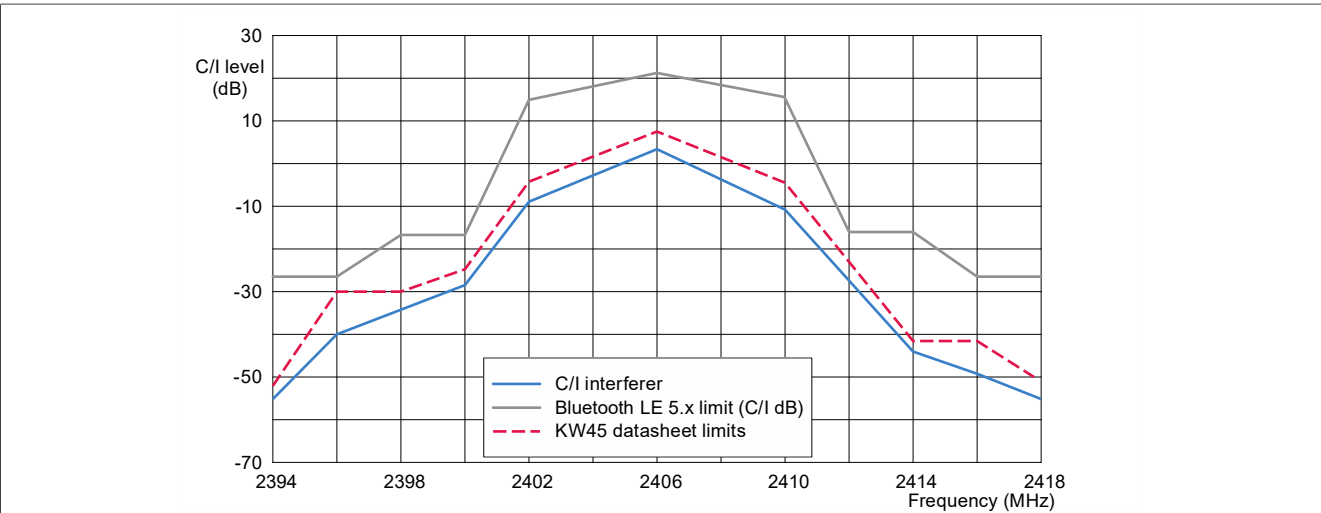
Figure 69. Adjacent, alternate, and co-channel rejection Bluetooth LE @ 2 Msps channel 2
