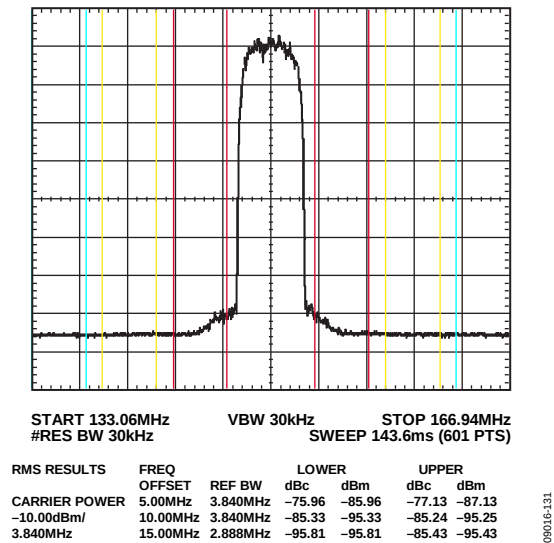
Figure 34. Four-Carrier W-CDMA ACLR Performance, IF ≈ 150 MHz
