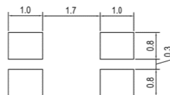
Figure 2) Suggested Land Pattern
