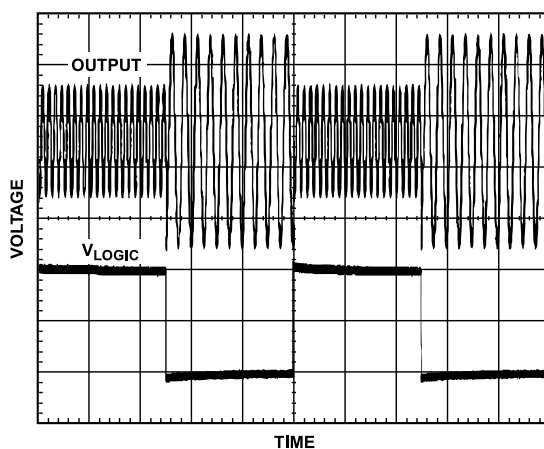
Figure 101. Multiplexed Output
