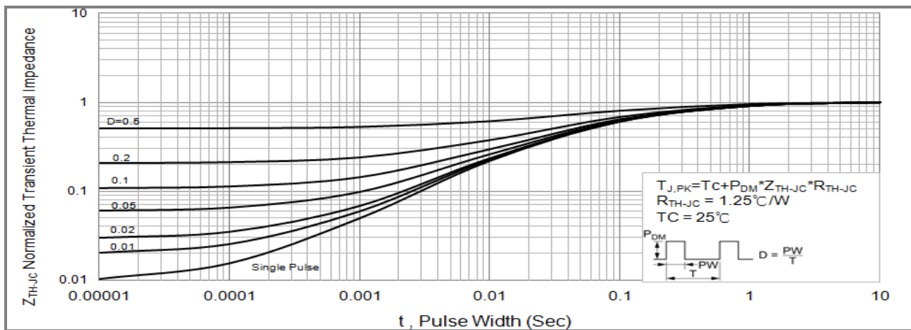
Fig.14 PJP4NA60 Normalized Transient Thermal Impedance vs. Pulse Width
