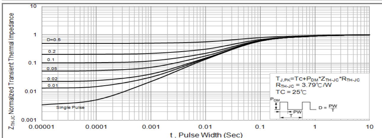
Fig.15 PJF4NA60 Normalized Transient Thermal Impedance vs. Pulse Width
