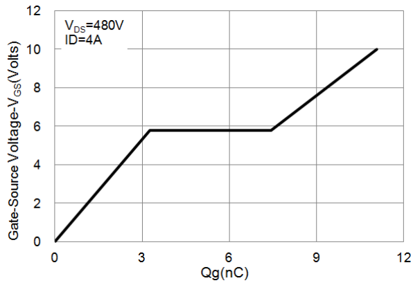
Fig.7 Gate Charge
