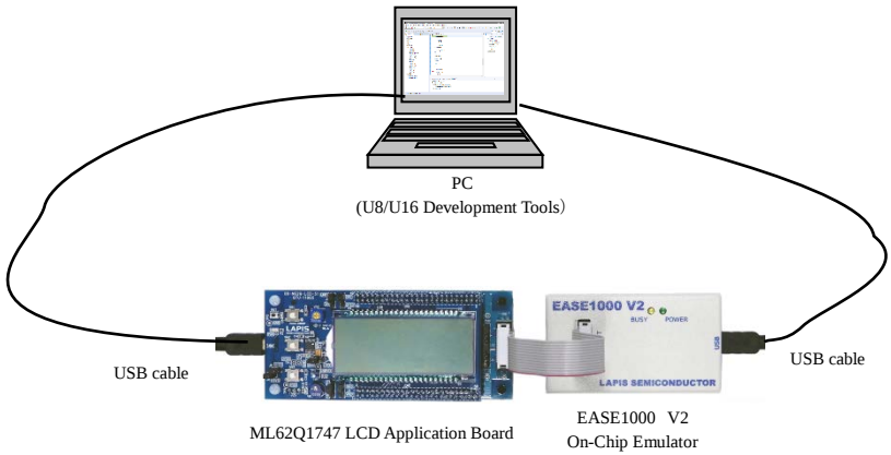
Figure 5 Use with the U8/U16 Development Tools configuration
