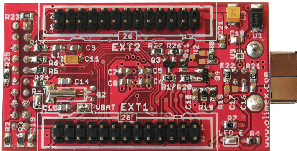
extension header 2
