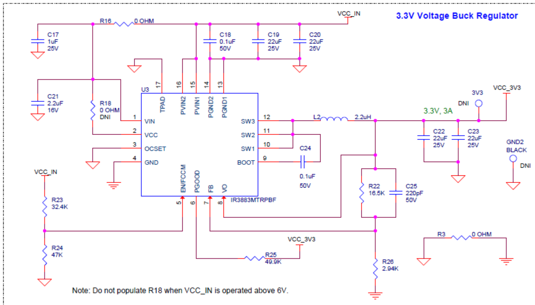
Figure 15 Power Supply - 2
