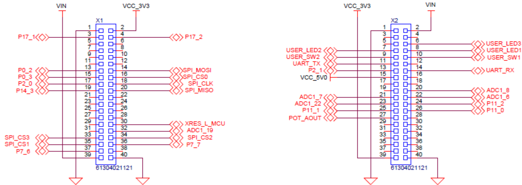
Figure 28 Shield2Go /MikroBUS
