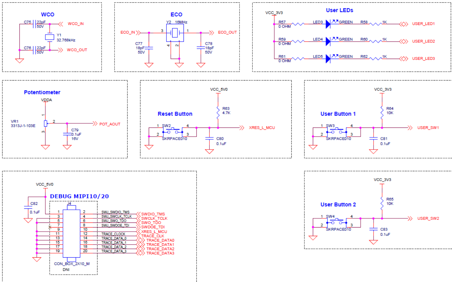
Figure 23 Peripheral Interface
