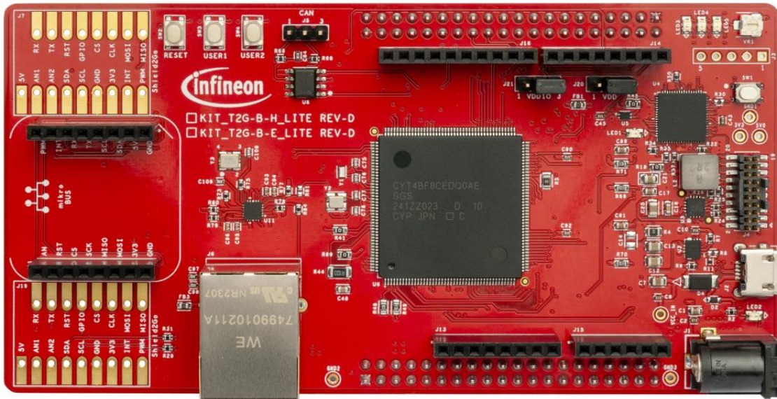
Figure 29 Top view
