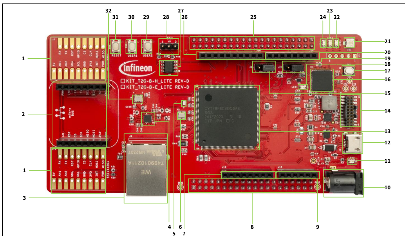
Figure 2 KIT_T2G-B-H_LITE board – top view
