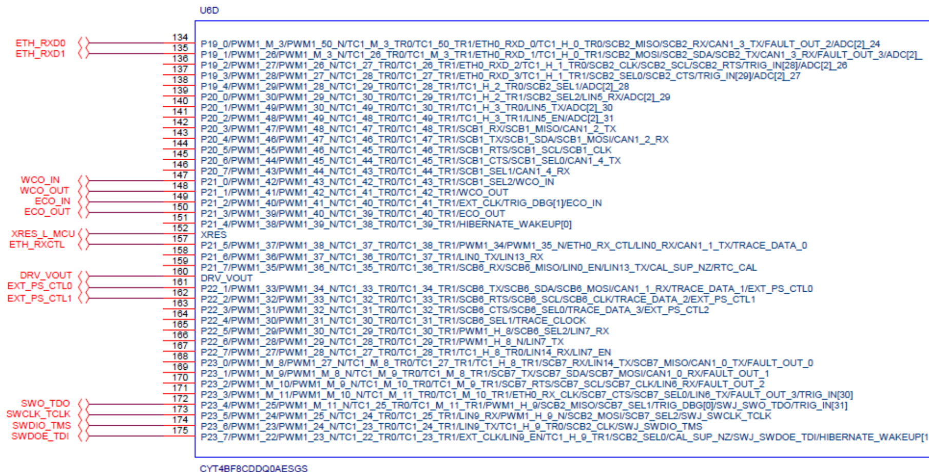
Figure 21 TRAVEO T2G-B-H-8M 176-pin MCU - 4
