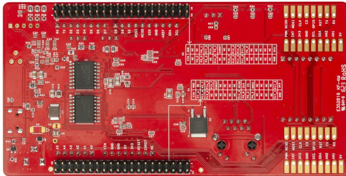
Figure 30 Bottom view
