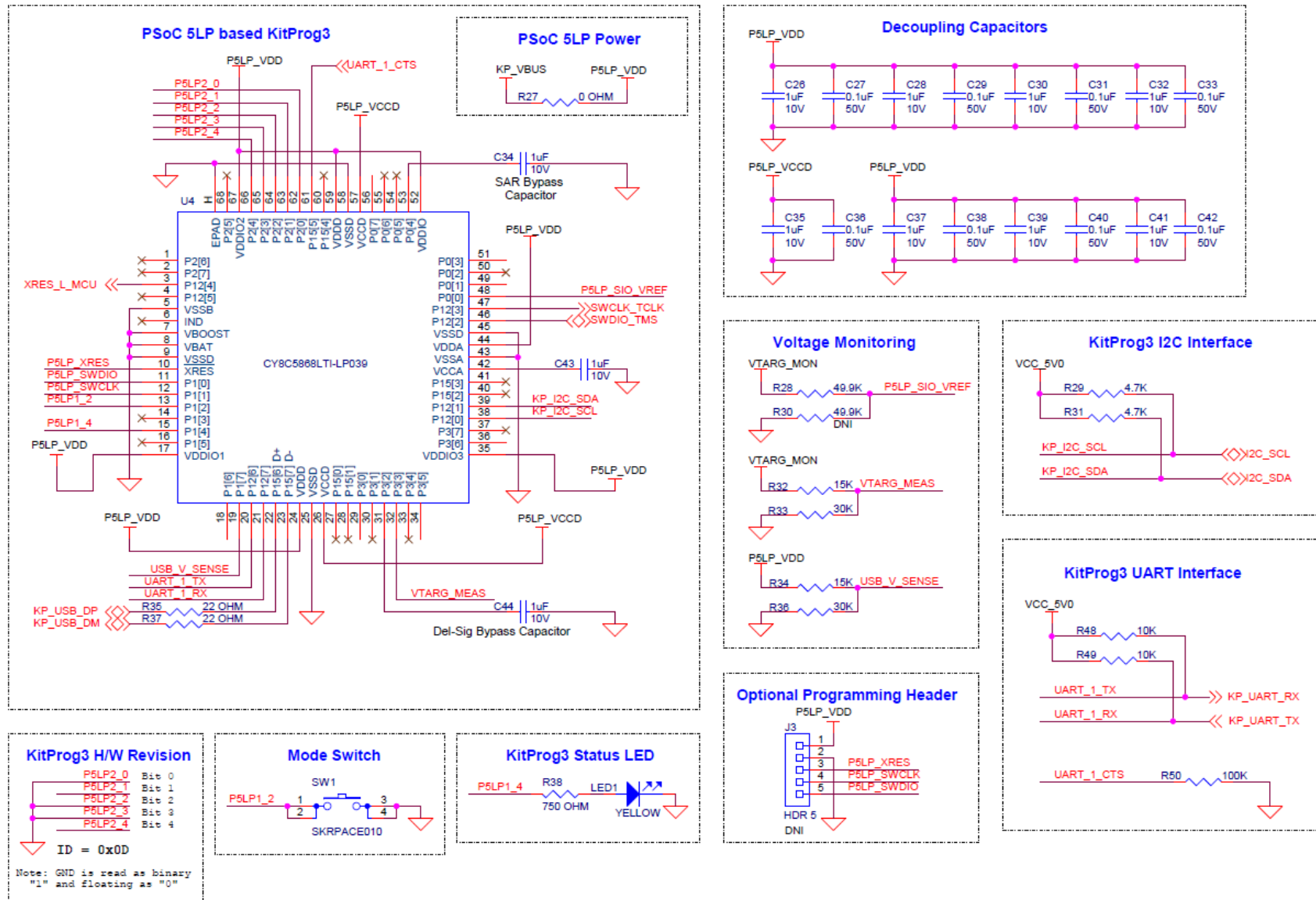
Figure 16 KitProg3 Interface
