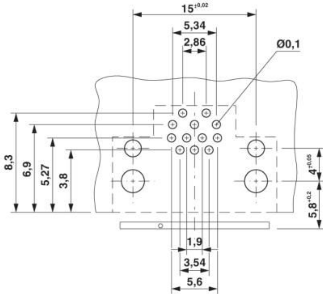
Drilling diagram
