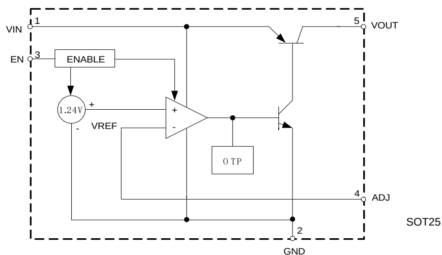
Adjustable Version
