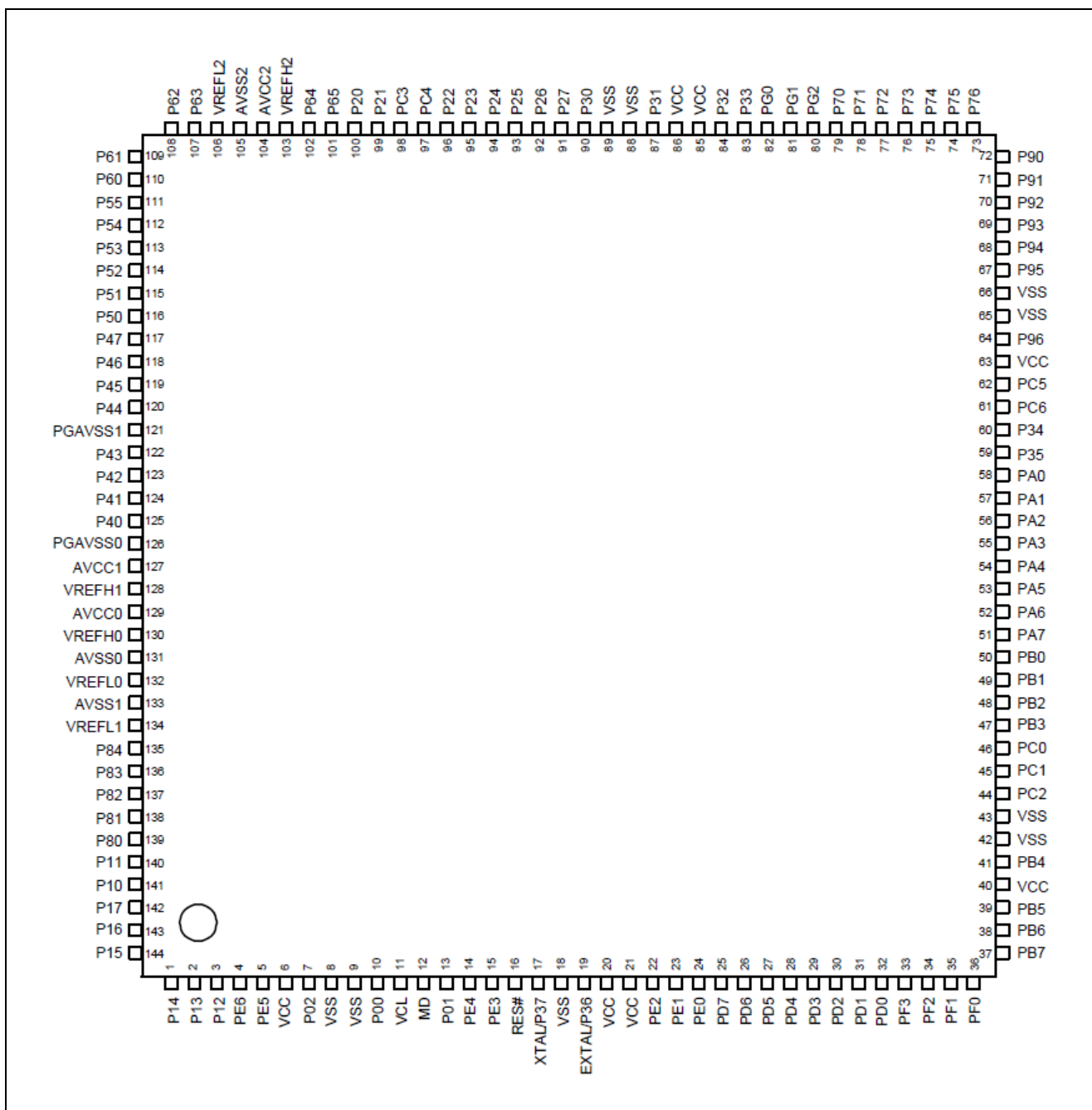
Figure 6.1 RX24U Pin Assignments
