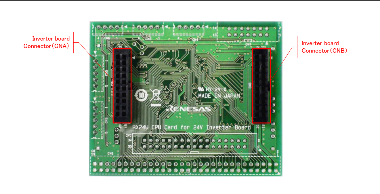
Figure 3.2 RX24U CPU Card Layout (Bottom View)
