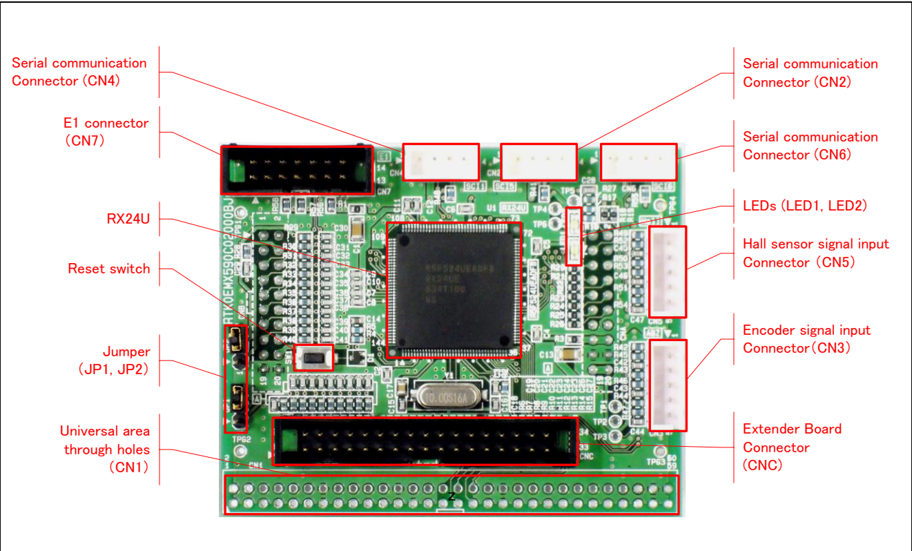
Figure 3.1 RX24U CPU Card Layout (Top View)
