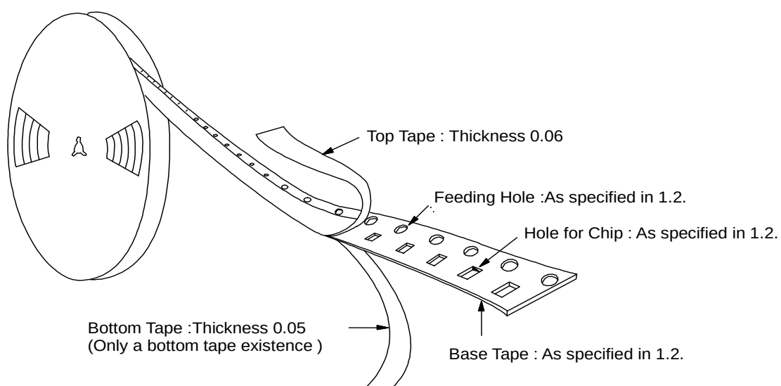
Fig.3 Taping Diagram
