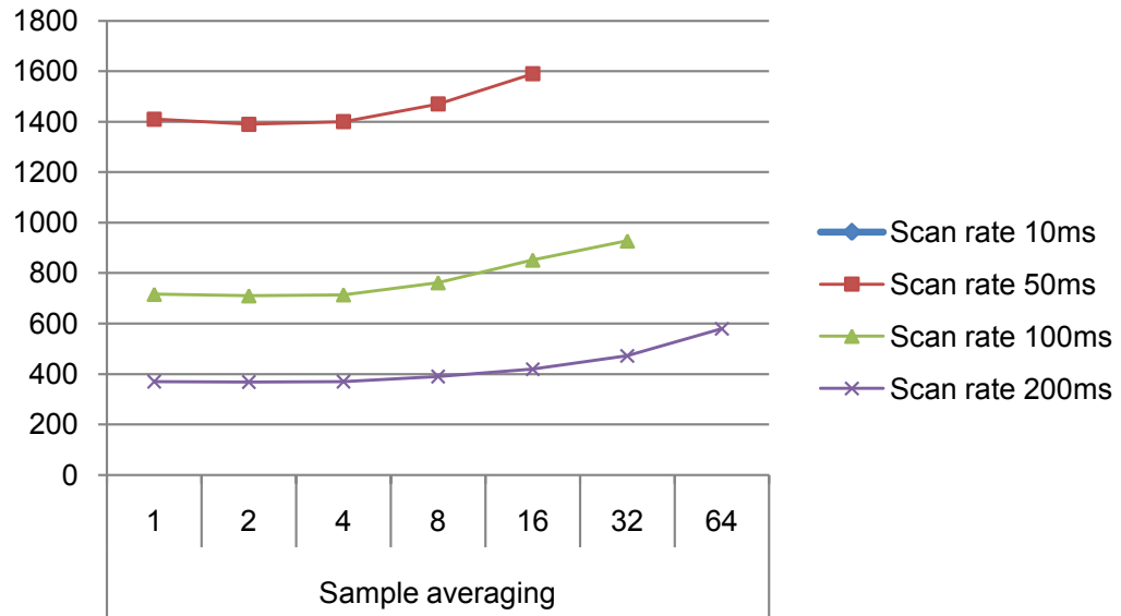
Figure 37-13. CPU Utilization
