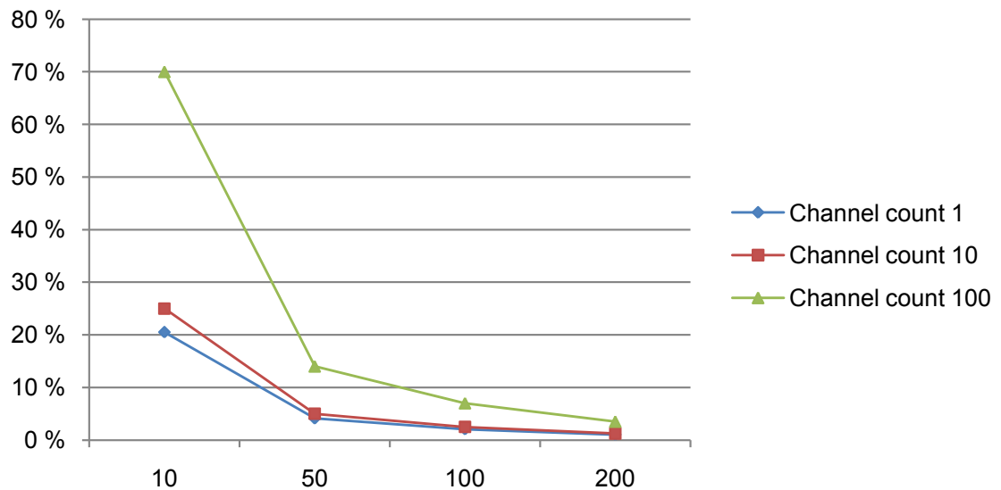
Figure 37-13. CPU Utilization
