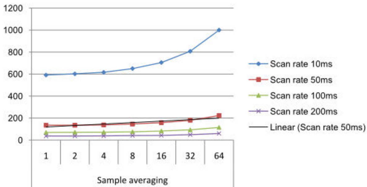
Figure 37-9. Power Consumption [ \mu\text{A} ] 10 sensors, noise countermeasures disabled, f=48\text{MHz} , V_{cc}=3.3\text{V}
