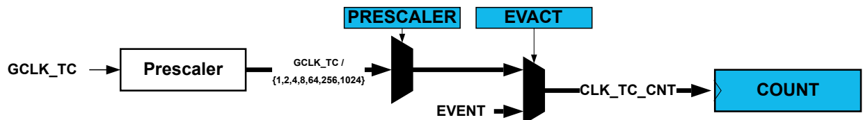
Figure 30-2. Prescaler
