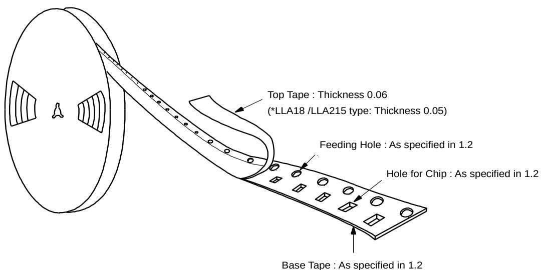
Fig3 Taping Diagram
