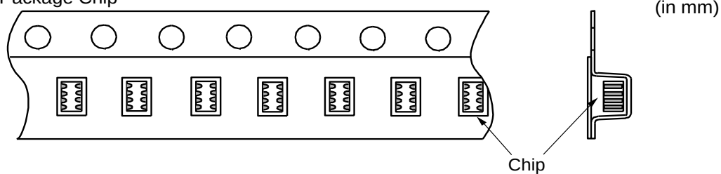
Fig.2 Dimension of Reel
