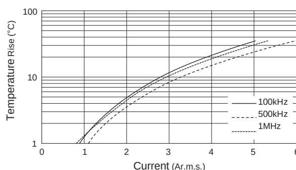
Ripple Current
