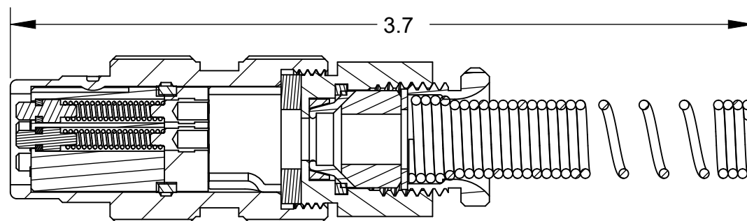
SECTION Z-Z
