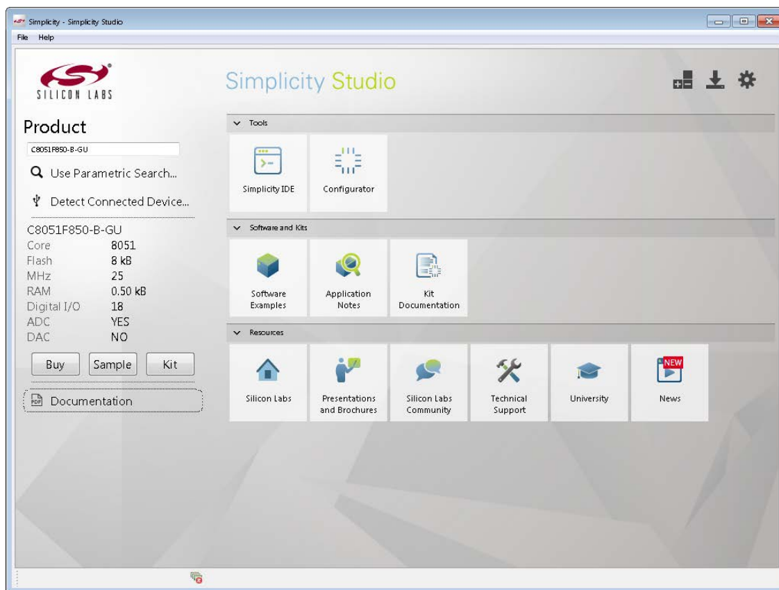
Figure 2. Simplicity Studio
