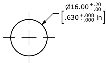
PANEL CUTOUT MAX. PANEL THICKNESS 10mm
