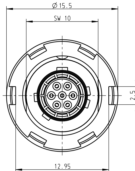
G80YAR-PO7WCD0-000L Mechanical coding: A Color Coding: light brown
