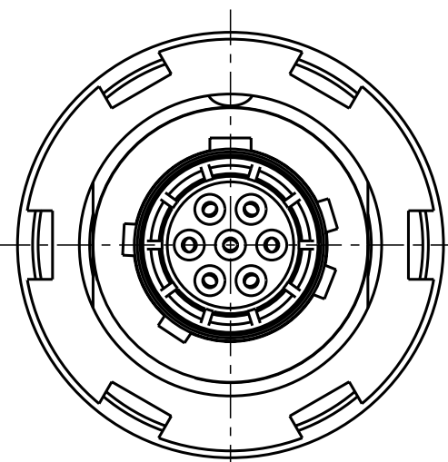
G80YCR-P07WCD0-000L Mechanical coding: C Color Coding: blue
