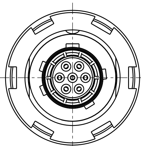
G80YDR-P07WCD0-000L Mechanical coding: D Color Coding: green
