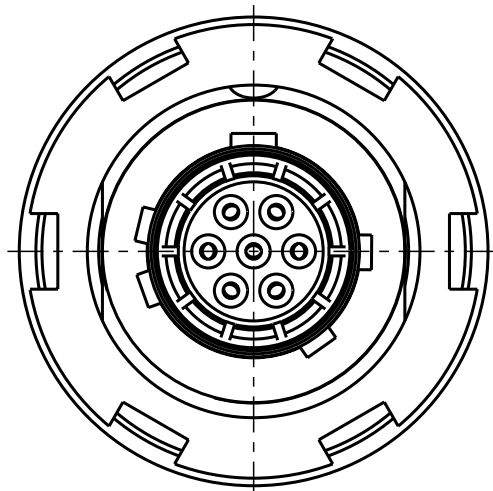
G80YBR-P07WCD0-000L Mechanical coding: B Color Coding: red
