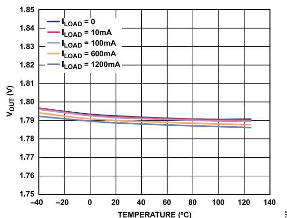
Figure 14. Output Voltage ( V_{OUT} ) vs. Temperature at Various Loads, V_{OUT} = 1.8\text{ V}
