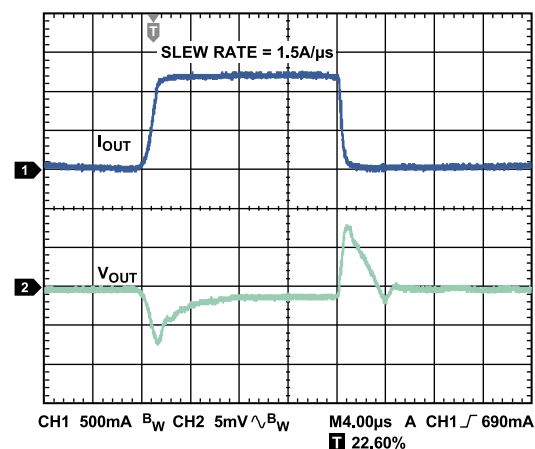
Figure 33. Load Transient Response, I_{LOAD} = 100 \text{ mA} to 1.2 \text{ A} , V_{OUT} = 3.3 \text{ V} , V_{IN} = 4.0 \text{ V} , C_{OUT} = 22 \mu\text{F} , Channel 1 = I_{OUT} , Channel 2 = V_{OUT}
