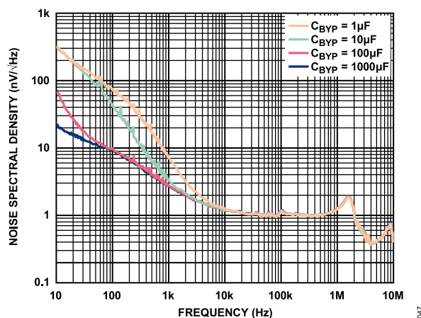
Figure 44. Noise Spectral Density vs. Frequency at Various C_{\text{BYP}} Values
