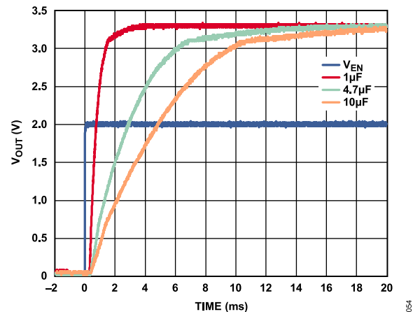
Figure 51. Typical Start-Up Behavior with C_{BYP} = 1 \mu F to 10 \mu F
