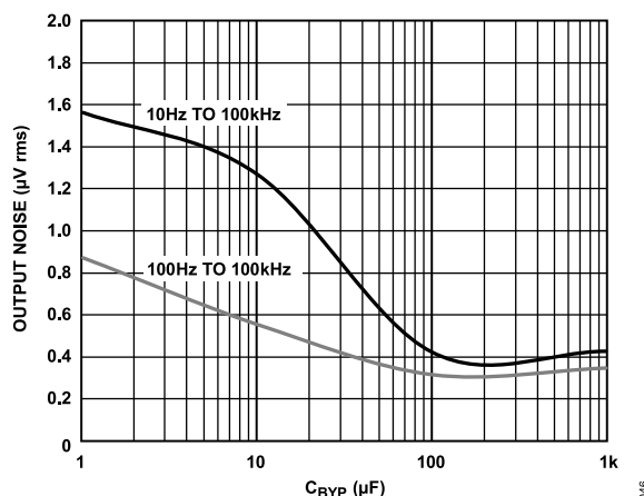
Figure 43. RMS Output Noise vs. Bypass Capacitance ( C_{\text{BYP}} )
