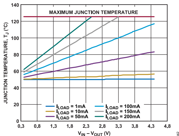
Figure 50. TSOT 50 \text{mm}^2 of PCB Copper, T_A = 50^{\circ}\text{C}
