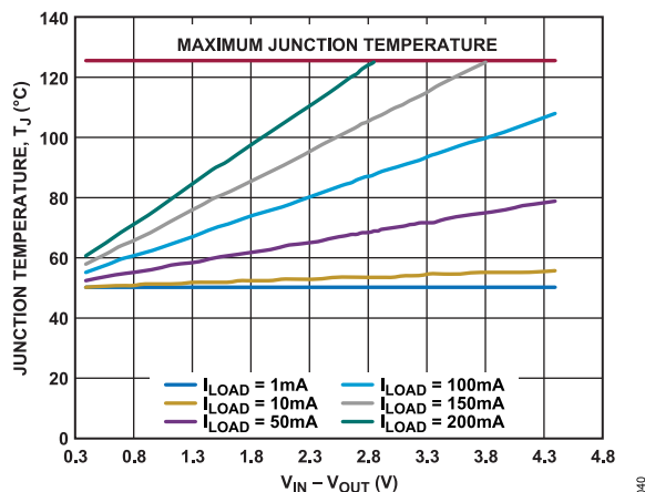
Figure 48. TSOT 500 \text{mm}^2 of PCB Copper, T_A = 50^{\circ}\text{C}
