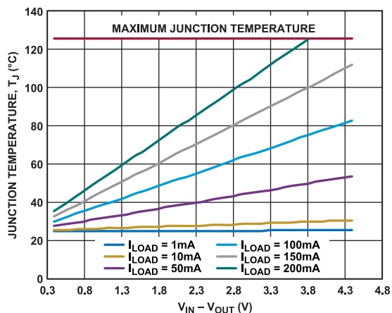
Figure 45. TSOT 500 \text{mm}^2 of PCB Copper, T_A = 25^{\circ}\text{C}
