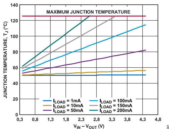
Figure 49. TSOT 100 \text{mm}^2 of PCB Copper, T_A = 50^{\circ}\text{C}
