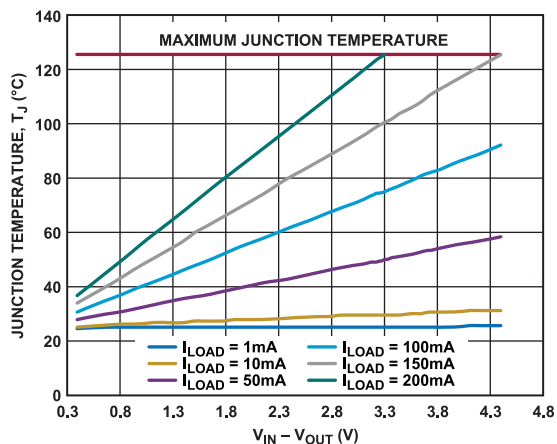
Figure 47. TSOT 50 \text{mm}^2 of PCB Copper, T_A = 25^{\circ}\text{C}
