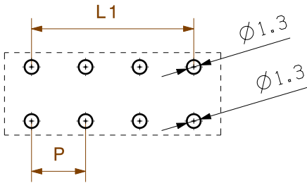
HOLE PATTERN
